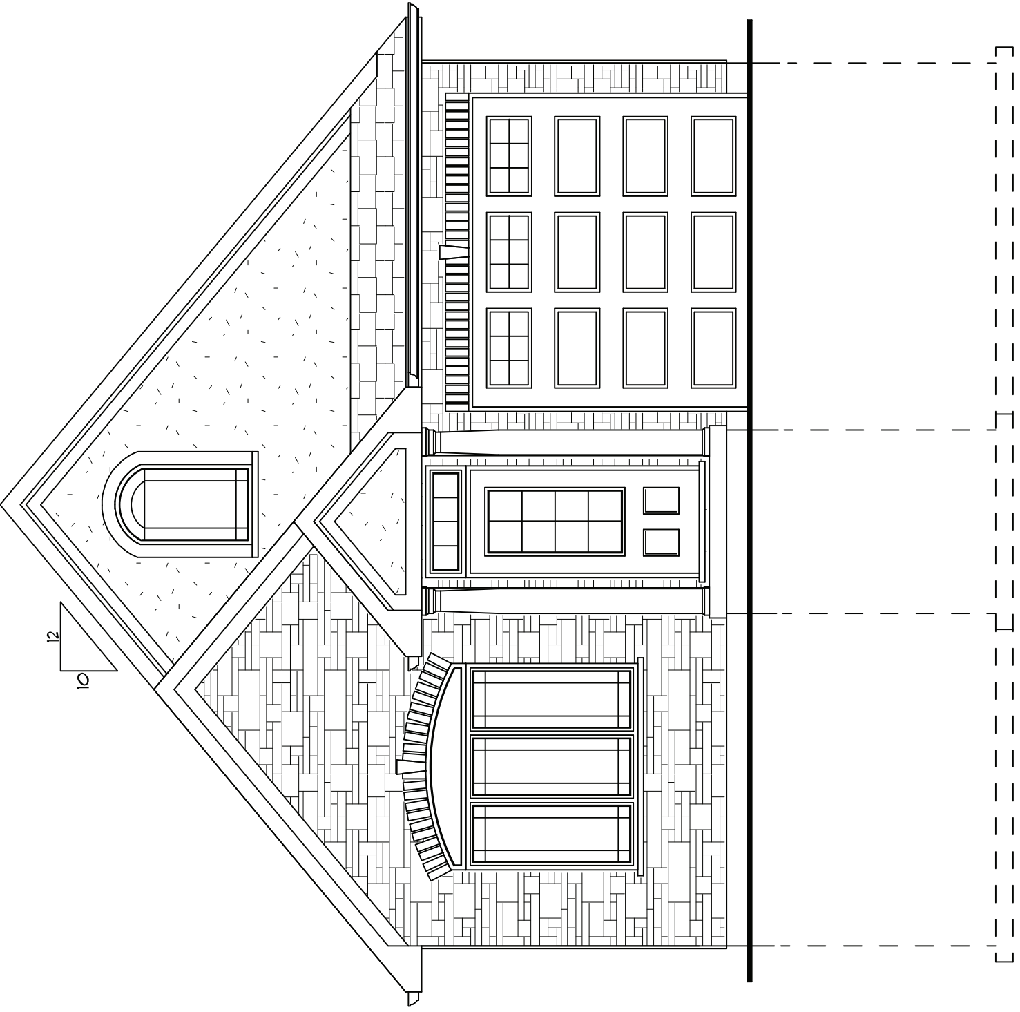
FRONT ELEVATION (OPT. B)
