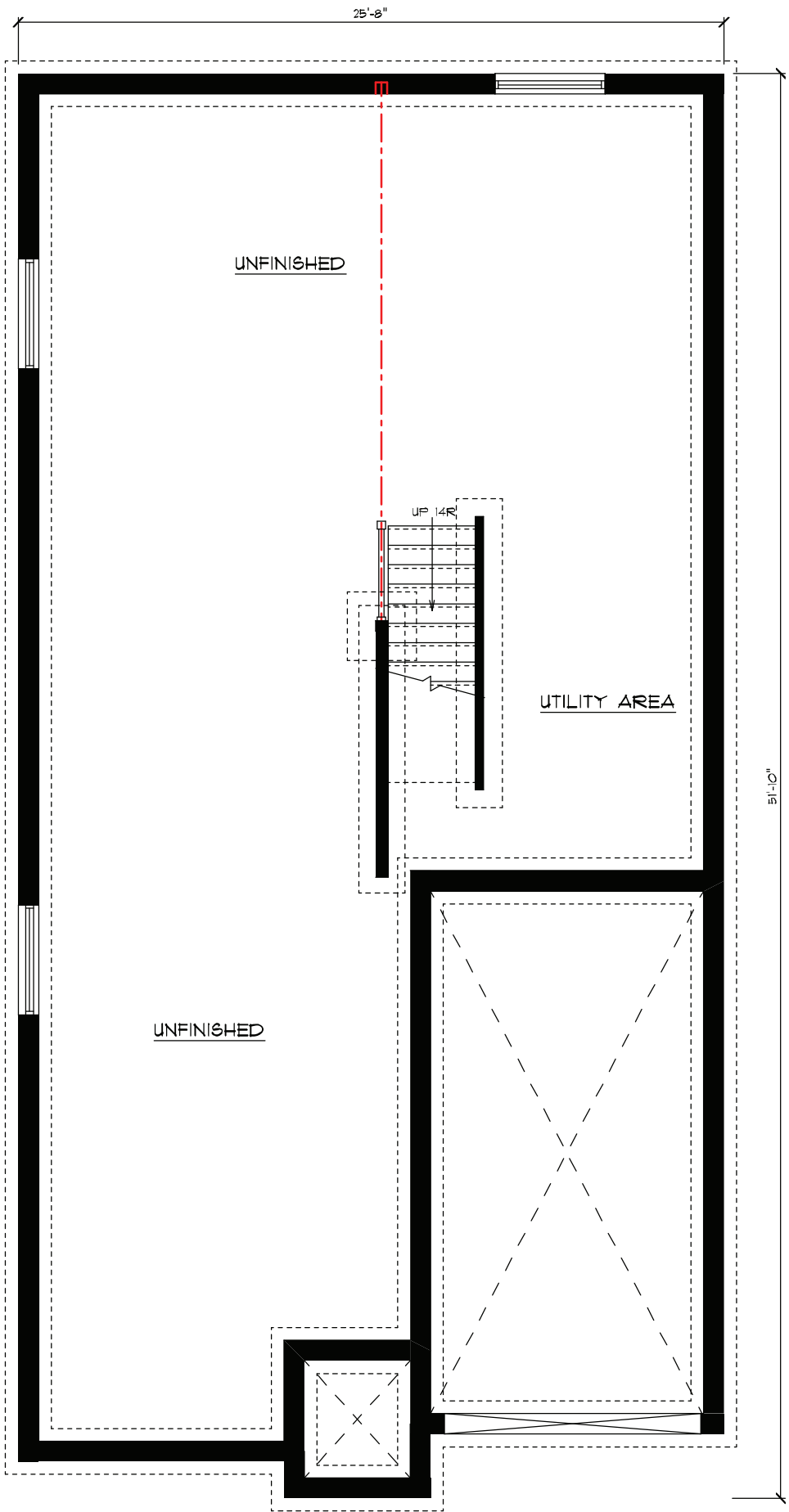
FOUNDATION PLAN
