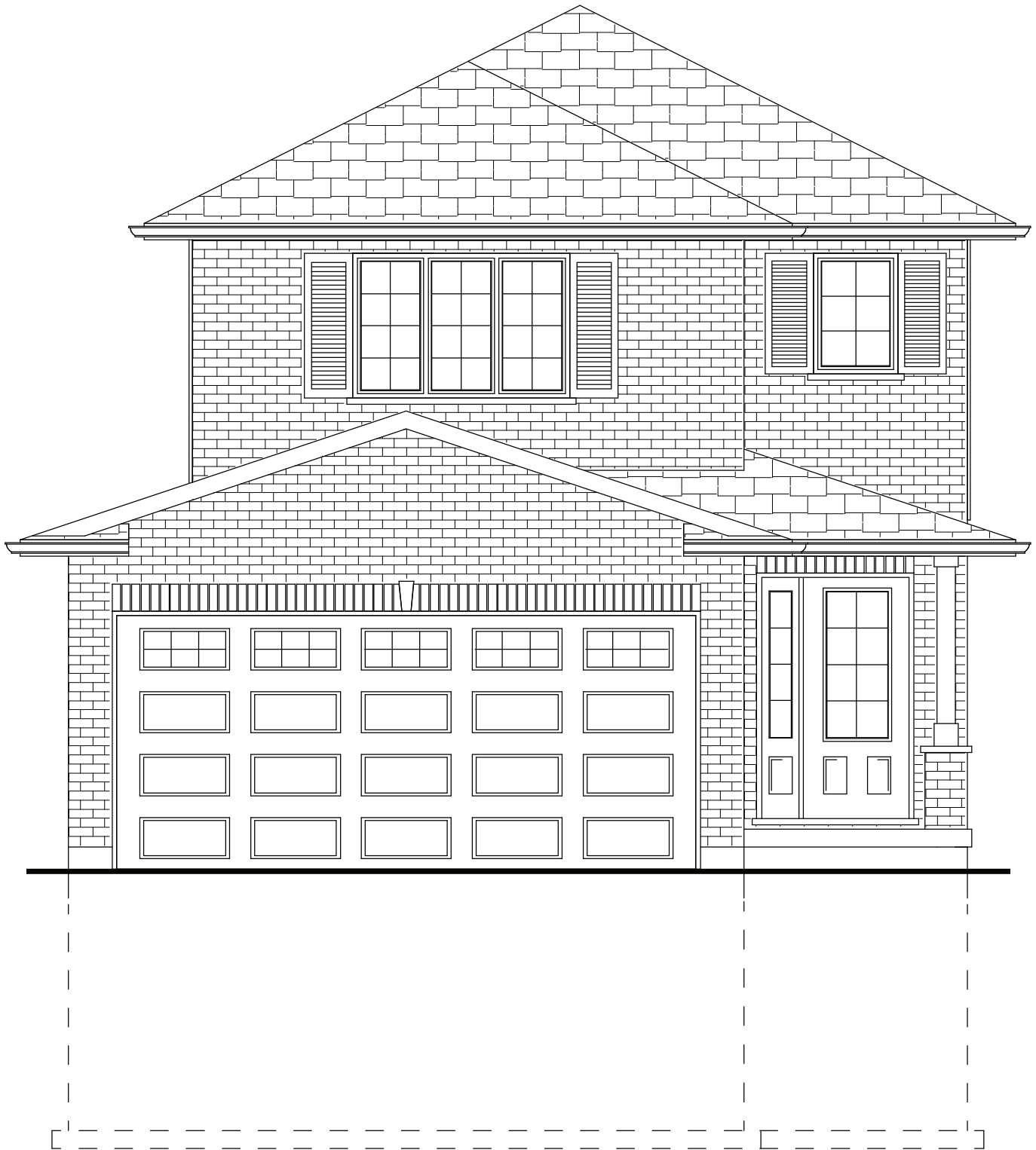
FRONT ELEVATION
